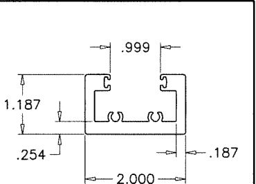
2R RAILING BOTTOM/SIDE FRAME
