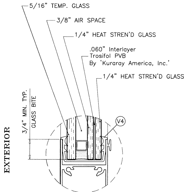
S.G.D. GLASS TYPE 'A' 1-1/4" OVERALL INSUL. LAM. GLASS
