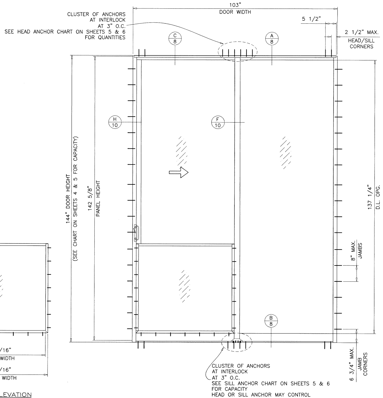
TYPICAL ELEVATION TESTED UNIT (XO WITH RAILING)
