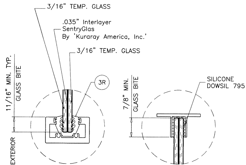
RAILING GLASS TYPE 'C' 7/16" NOMINAL LAM. GLASS
