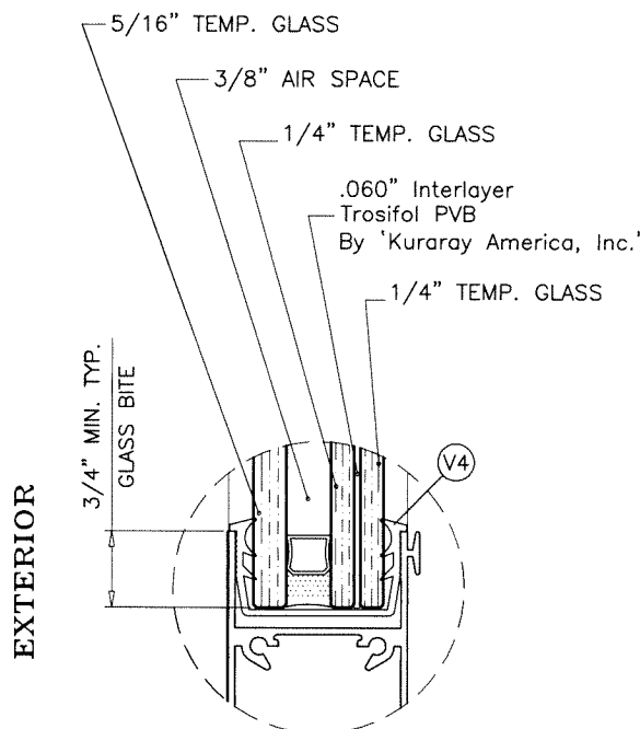
S.G.D. GLASS TYPE 'B' 1-1/4" OVERALL INSUL. LAM. GLASS
